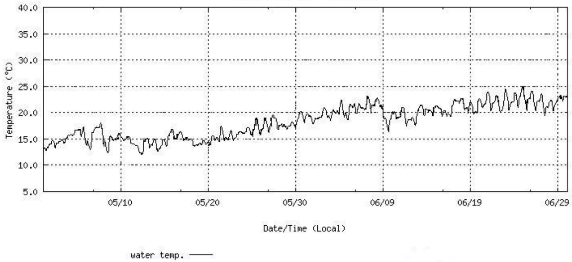
NOAA/NOS/CO-OPS Air/Water Temperature Plot 8557380 Lewes, DE from 2010/05/01 - 2010/06/30
